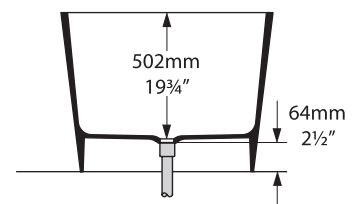
Section BB Shown with K12/K40 waste kit
