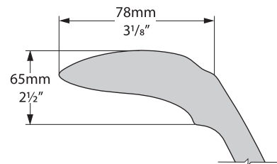
Rim detail
